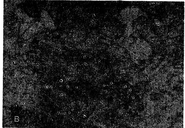
Figure A s Mcrophoto of hornblende-gabbro showing albite and carlsbad twinned plagioclase crystals. idiomorphic and hypidiomorphic plagioclase faths show directional texture. Hornblendes are intergranular with plagioclase crystals. Sample no: 187» from SW of Çamsan, x nicöi, x35.
